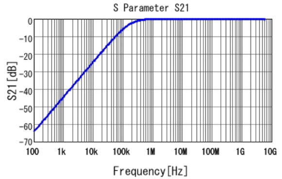
■ GRT155R71E103KE01 S21 DC0V, 25degC
