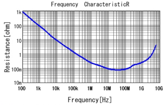
■ GRT155R71E103KE01 R DC0V, 25degC
