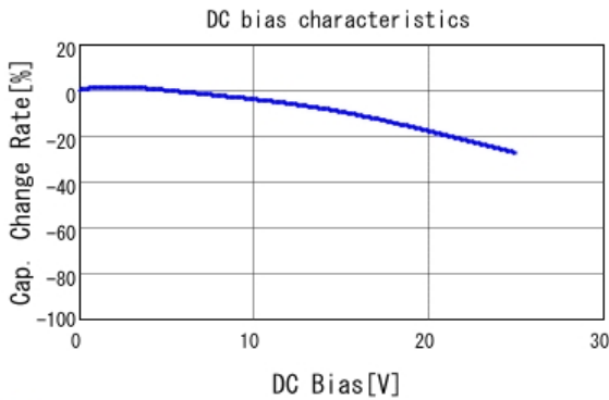
■ GRT155R71E103KE01 C-DC bias capchange, 25.0degC, AC1.
