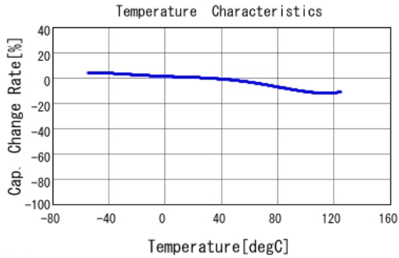
■ GRT155R71E103KE01 C-Temp. capchange, DC0.0V, AC1.0Vrm
