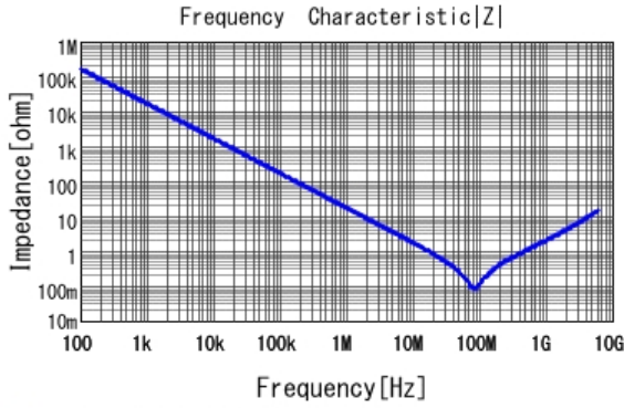
■ GRT155R71E103KE01 |Z| DC0V, 25degC
