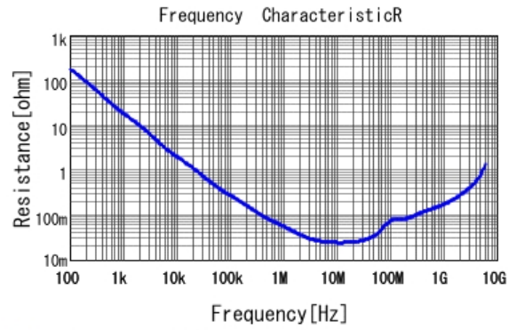
■ GRT155R71C473KE01 R DCOV, 25degC
