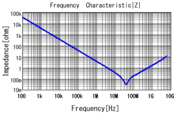
■ GRT155R71C473KE01 |Z| DCOV, 25degC
