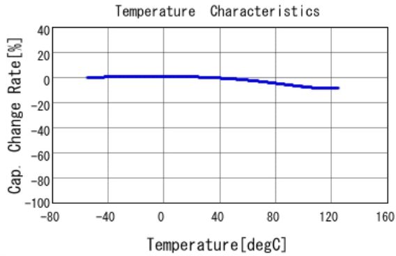
■ GRT155R71C473KE01 C-Temp. capchange, DC0.0V, AC1.0Vrm
