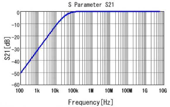
■ GRT155R71C473KE01 S21 DC0V, 25degC
