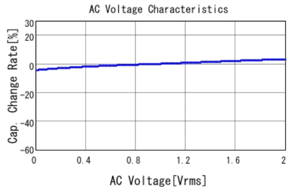
■ GRT155R71C473KE01 C-AC Voltage capchange, DCOV, 25.0d
