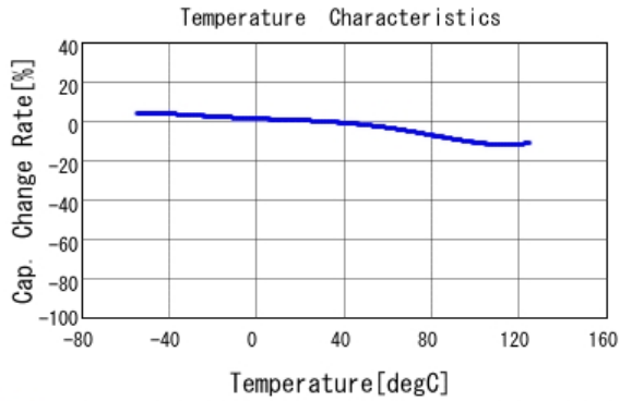
■ GRT155R71C103KE01 C-Temp. capchange, DC0.0V, AC1.0Vrm
