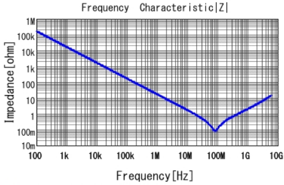
■ GRT155R71C103KE01 |Z| DCOV, 25degC
