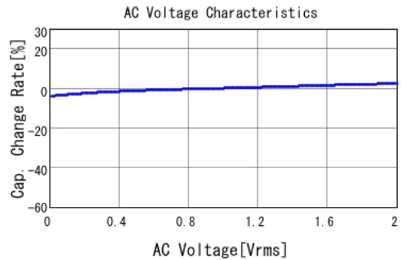
■ GRT155R71C103KE01 C-AC Voltage capchange, DCOV, 25.0d
