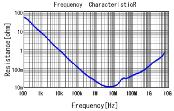
■ GRT155R70J105KE01 R DC0V, 25degC
