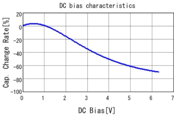
■ GRT155R70J105KE01 C-DC bias capchange, 25.0degC, AC0.
