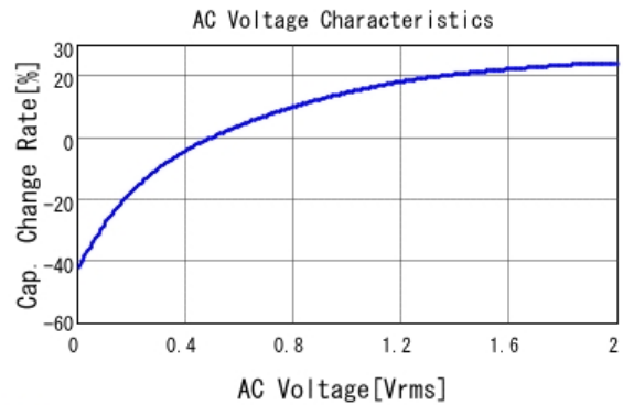
■ GRT155R70J105KE01 C-AC Voltage capchange, DC0V, 25.0d
