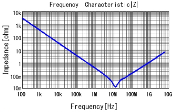
■ GRT155R70J105KE01 |Z| DC0V, 25degC
