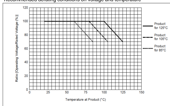
Recommended derating conditions on voltage and temperature
