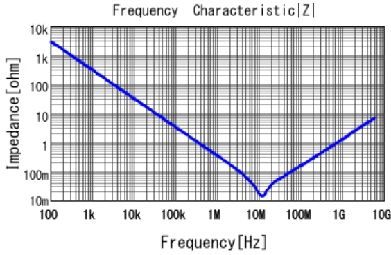
■ GRT155R61E105KE01 |Z| DC0V, 25degC
