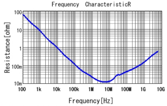
■ GRT155R61E105KE01 R DC0V, 25degC
