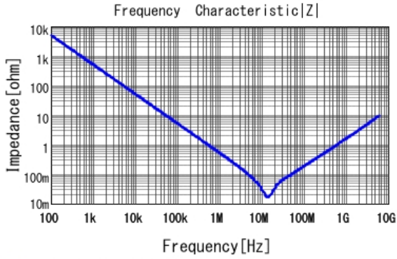
■ GRT155R61A334KE01 |Z| DCOV, 25degC
