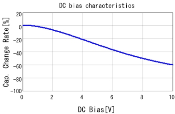
■ GRT155R61A334KE01 C-DC bias capchange, 25.0degC, AC0.
