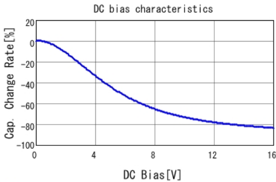
■ GRT155C81C105KE13 C-DC bias capchange, 25.0degC, AC1V
