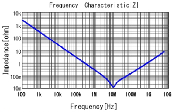
■ GRT155C81C105KE13 |Z| DCOV, 25degC
