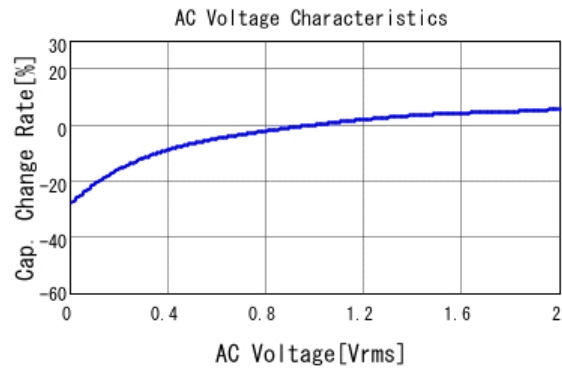
■ GRT155C81C105KE13 C-AC Voltage capchange, DCOV, 25.0d
