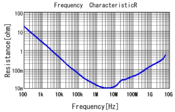
■ GRT155C81C105KE13 R DCOV, 25degC
