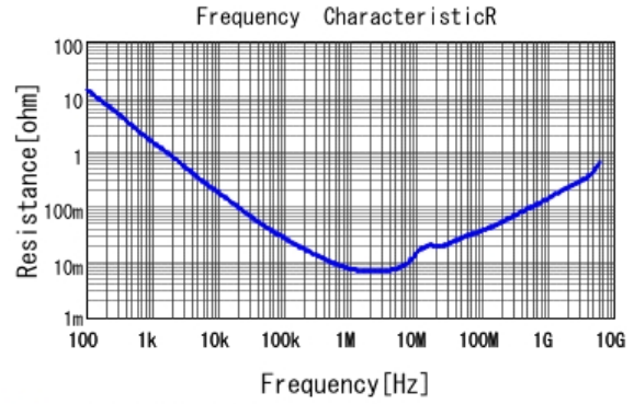
■ GRT155C81A225KE13 R DCOV, 25degC
