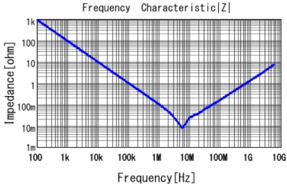
■ GRT155C81A225KE13 |Z| DCOV, 25degC
