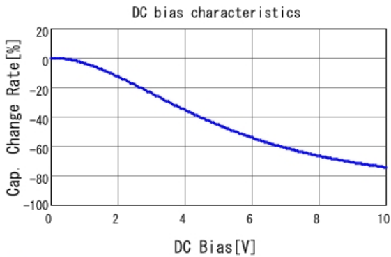
■ GRT155C81A225KE13 C-DC bias capchange, 25.0degC, AC1V
