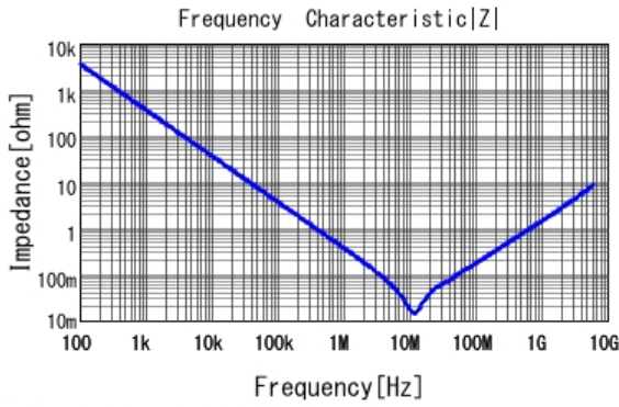
■ GRT155C80J474KE01 |Z| DCOV, 25degC
