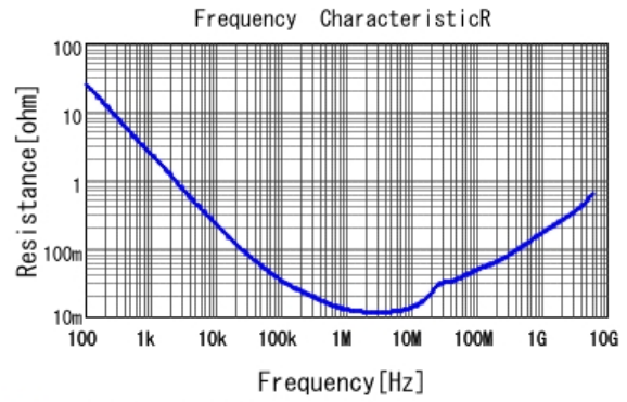
■ GRT155C80J474KE01 R DCOV, 25degC
