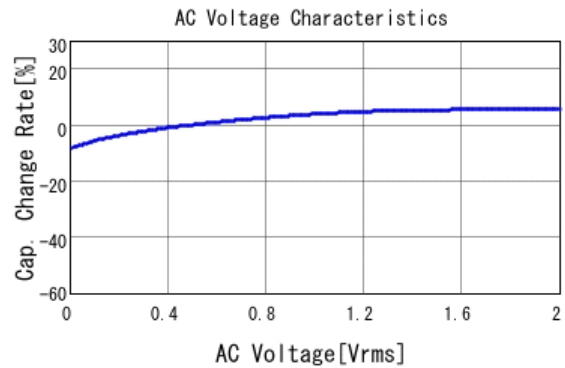
■ GRT155C80J474KE01 C-AC Voltage capchange, DCOV, 25.0d
