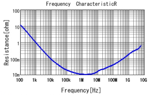
■ GRT155C80J225KE01 R DC0V, 25degC
