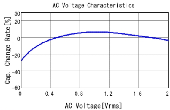
■ GRT155C80J225KE01 C-AC Voltage capchange, DC0V, 25.0d
