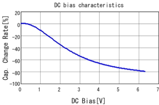
■ GRT155C80J225KE01 C-DC bias capchange, 25.0degC, AC0.
