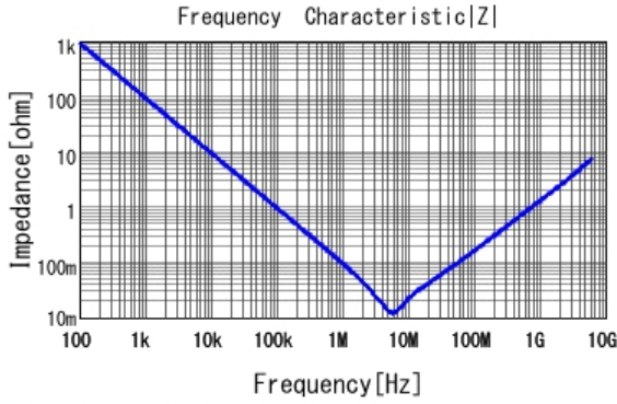
■ GRT155C80J225KE01 |Z| DC0V, 25degC
