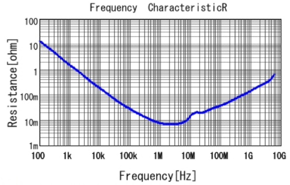
■ GRT155C71A225KE13 R DCOV, 25degC
