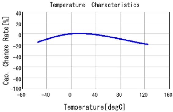
■ GRT155C71A225KE13 C-Temp. capchange, DC0.0V, AC0.1Vrm
