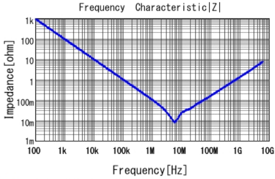
■ GRT155C71A225KE13 |Z| DCOV, 25degC
