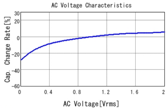
■ GRT155C71A105KE13 C-AC Voltage capchange, DCOV, 25.0d
