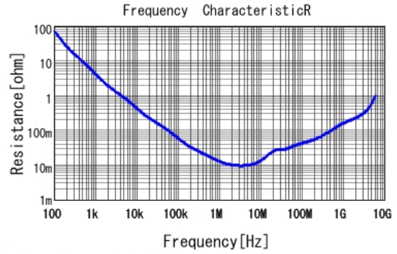
■ GRT155C71A105KE13 R DCOV, 25degC
