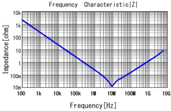
■ GRT155C71A105KE13 |Z| DCOV, 25degC
