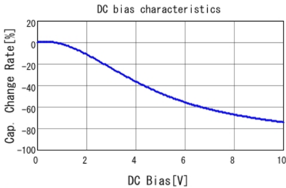
■ GRT155C71A105KE13 C-DC bias capchange, 25.0degC, AC1V
