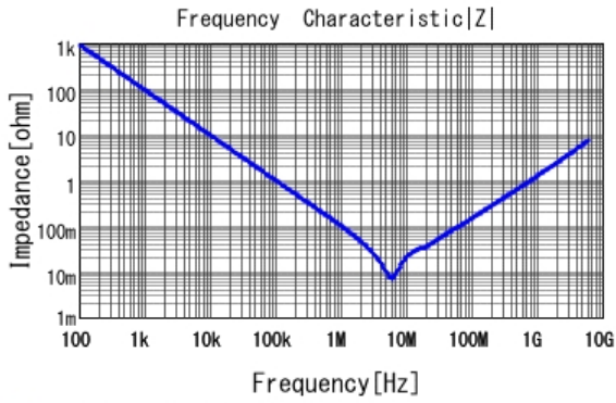
■ GRT155C70J225KE13 |Z| DCOV, 25degC
