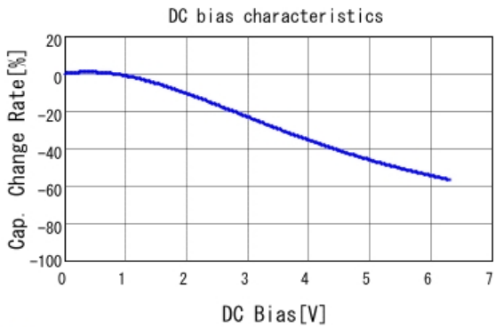
■ GRT155C70J225KE13 C-DC bias capchange, 25.0degC, AC0.
