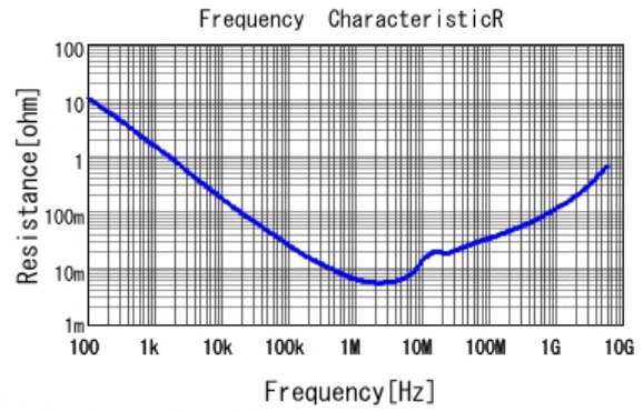
■ GRT155C70J225KE13 R DCOV, 25degC
