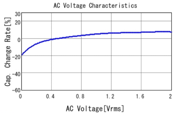
■ GRT155C70J225KE13 C-AC Voltage capchange, DCOV, 25.0d
