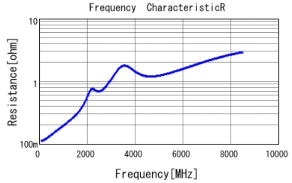
■ GRT1555C2A820JA02 R DC0V, 25degC
