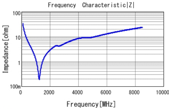
■ GRT1555C2A470JA02 |Z| DC0V, 25degC
