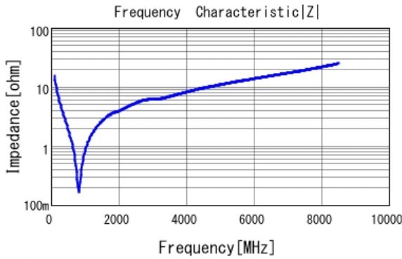
■ GRT1555C2A101JA02 |Z| DC0V, 25degC
