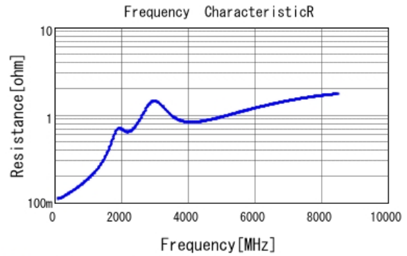
■ GRT1555C2A101JA02 R DC0V, 25degC
