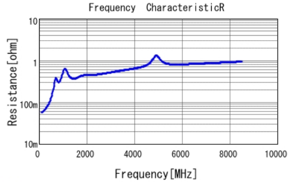
■ GRT1555C1H681JA02 R DCOV, 25degC
