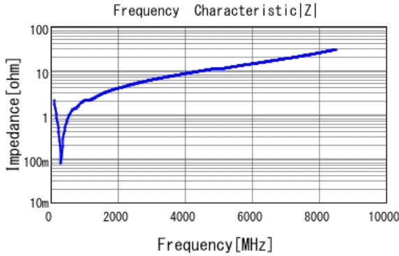
■ GRT1555C1H681JA02 |Z| DCOV, 25degC
