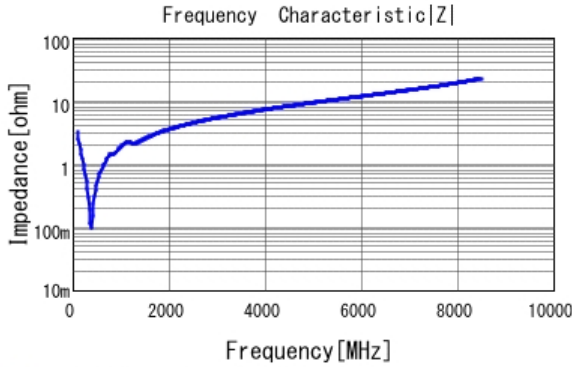
■ GRT1555C1E471JA02 |Z| DC0V, 25degC
