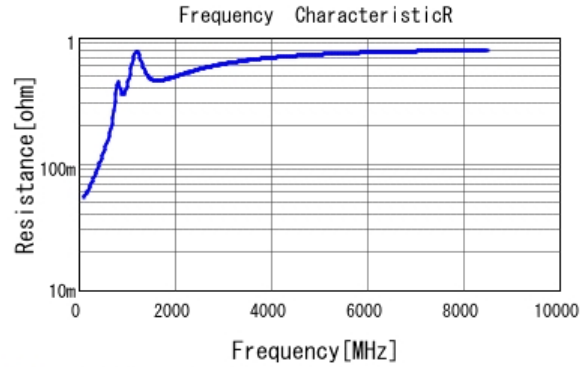
■ GRT1555C1E471JA02 R DC0V, 25degC
