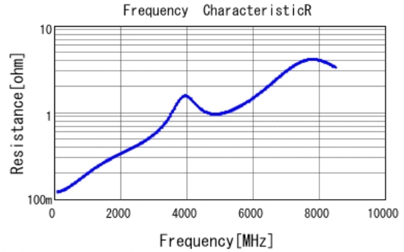
■ GRT1555C1E220JA02 R DC0V, 25degC
