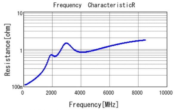
■ GRT1555C1E101JA02 R DC0V, 25degC
