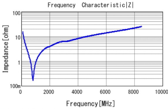
■ GRT1555C1E101JA02 |Z| DC0V, 25degC
