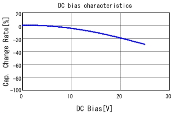
■ GRT033R71E102KE01 C-DC bias capchange, 25.0degC, AC1.
