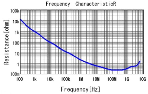
■ GRT033R71E102KE01 R DC0V, 25degC
