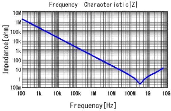
■ GRT033R71E102KE01 |Z| DC0V, 25degC
