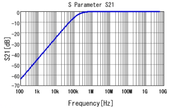
■ GRT033R71A103KE01 S21 DC0V, 25degC
