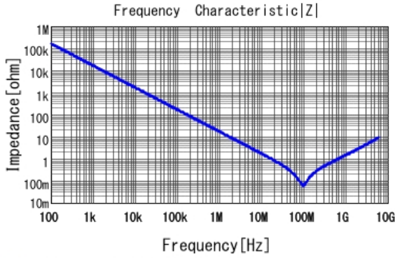
■ GRT033R71A103KE01 |Z| DCOV, 25degC
