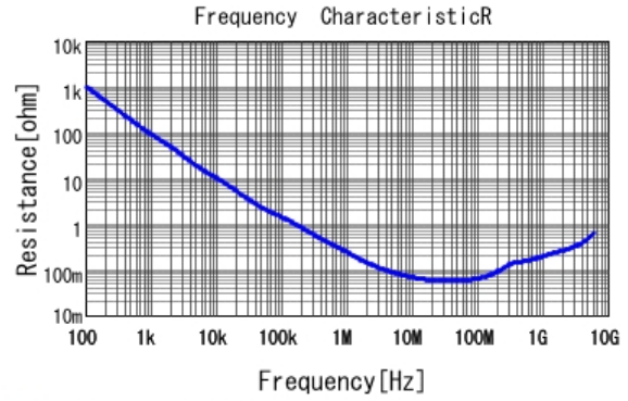
■ GRT033R71A103KE01 R DCOV, 25degC
