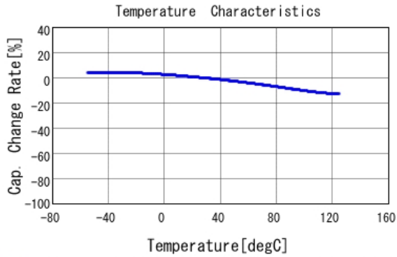
■ GRT033R71A103KE01 C-Temp. capchange, DC0.0V, AC1.0Vrm
