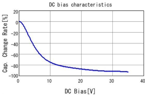
■ GRT033R6YA104KE01 C-DC bias capchange, 25.0degC, AC1V
