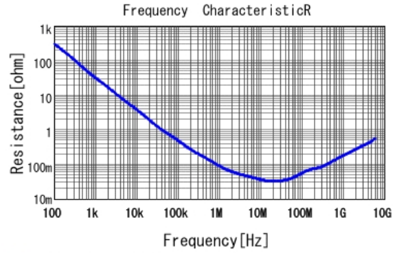
■ GRT033R6YA104KE01 R DCOV, 25degC
