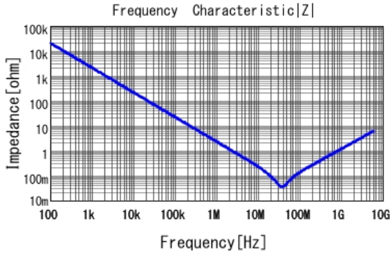
■ GRT033R6YA104KE01 |Z| DCOV, 25degC
