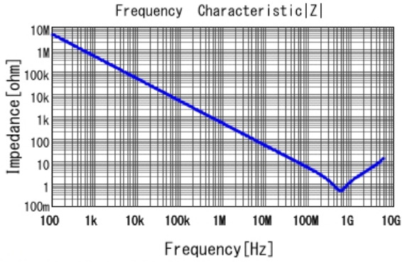
■ GRT033R61E331KE01 |Z| DCOV, 25degC
