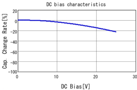
■ GRT033R61E331KE01 C-DC bias capchange, 25.0degC, AC1.
