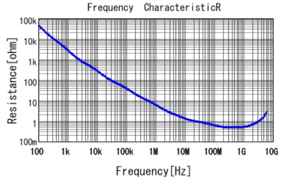
■ GRT033R61E331KE01 R DCOV, 25degC
