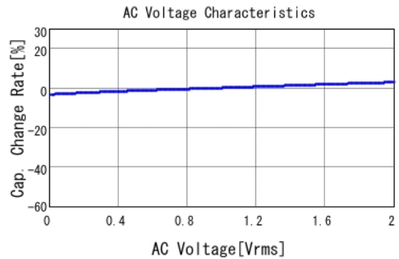
■ GRT033R61E331KE01 C-AC Voltage capchange, DCOV, 25.0d
