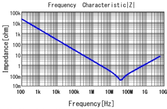
■ GRT033R61E104KE01 |Z| DC0V, 25degC
