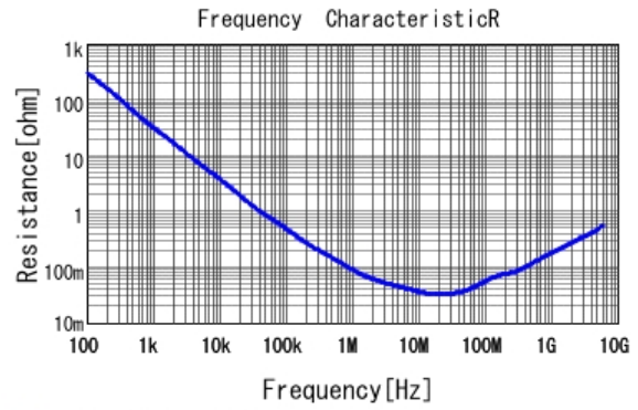
■ GRT033R61E104KE01 R DC0V, 25degC
