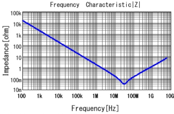
■ GRT033R61C104KE01 |Z| DCOV, 25degC
