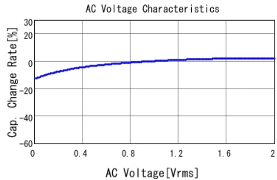
■ GRT033R61C104KE01 C-AC Voltage capchange, DCOV, 25.0d
