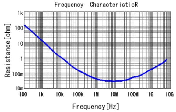
■ GRT033R61C104KE01 R DCOV, 25degC
