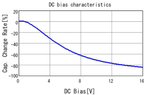
■ GRT033R61C104KE01 C-DC bias capchange, 25.0degC, AC1.
