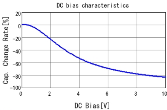
■ GRT033R61A224KE01 C-DC bias capchange, 25.0degC, AC0.
