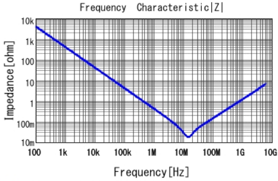
■ GRT033R60J474KE01 |Z| DC0V, 25degC
