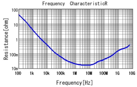
■ GRT033R60J474KE01 R DC0V, 25degC
