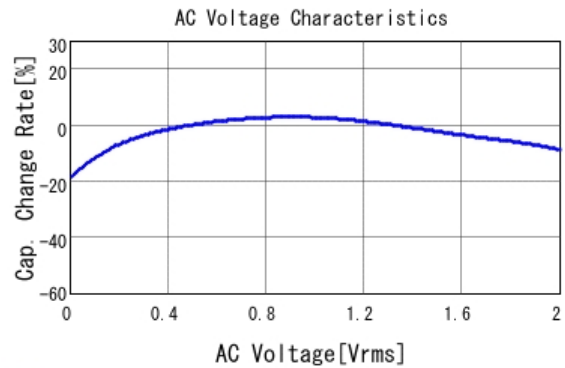
■ GRT033R60J474KE01 C-AC Voltage capchange, DC0V, 25.0d
