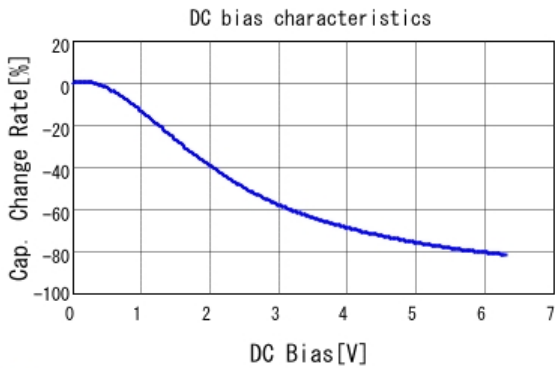
■ GRT033R60J474KE01 C-DC bias capchange, 25.0degC, AC0.
