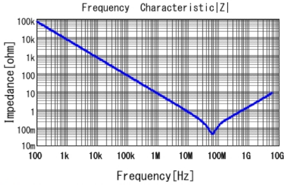
■ GRT033R60J223KE01 |Z| DCOV, 25degC
