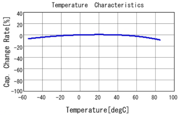
■ GRT033R60J223KE01 C-Temp. capchange, DC0.0V, AC0.5Vrm
