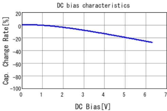
■ GRT033R60J223KE01 C-DC bias capchange, 25.0degC, AC0.
