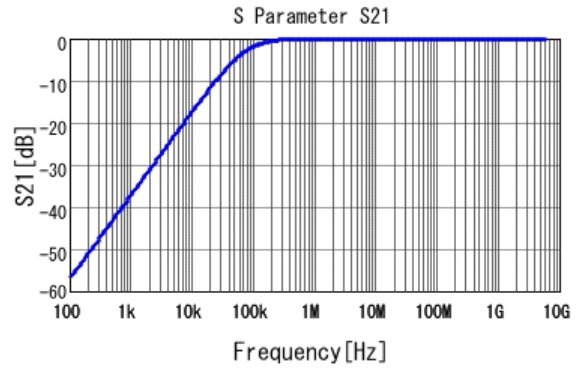
■ GRT033R60J223KE01 S21 DC0V, 25degC
