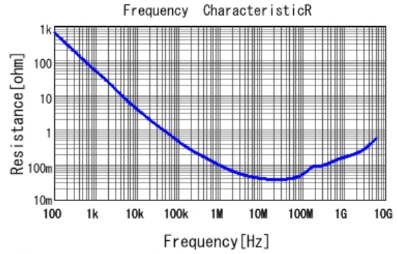
■ GRT033R60J223KE01 R DCOV, 25degC
