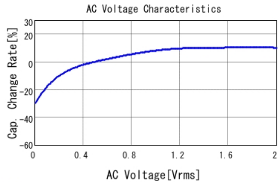
■ GRT033R60J104KE01 C-AC Voltage capchange, DCOV, 25.0d
