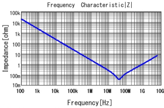
■ GRT033R60J104KE01 |Z| DCOV, 25degC
