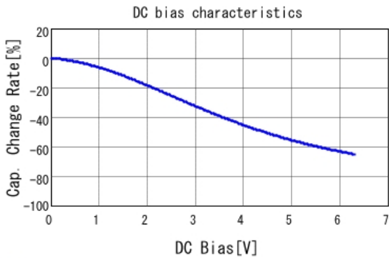
■ GRT033R60J104KE01 C-DC bias capchange, 25.0degC, AC0.
