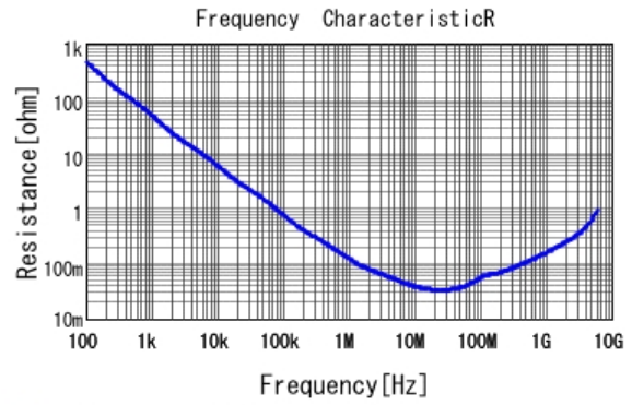
■ GRT033R60J104KE01 R DCOV, 25degC
