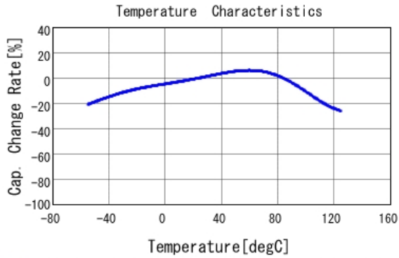
■ GRT033D70J105ME13 C-Temp. capchange, DC0.0V, AC0.02Vr
