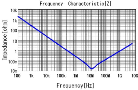
■ GRT033D70J105ME13 |Z| DCOV, 25degC
