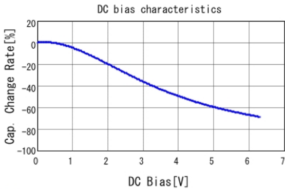
■ GRT033D70J105ME13 C-DC bias capchange, 25.0degC, AC0.
