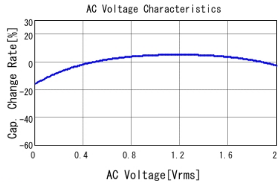
■ GRT033D70J105ME13 C-AC Voltage capchange, DCOV, 25.0d
