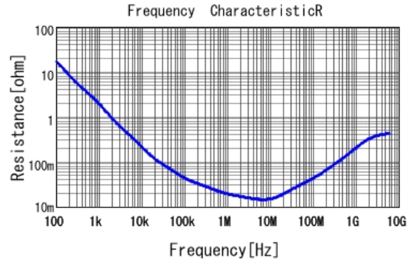
■ GRT033D70J105ME13 R DCOV, 25degC
