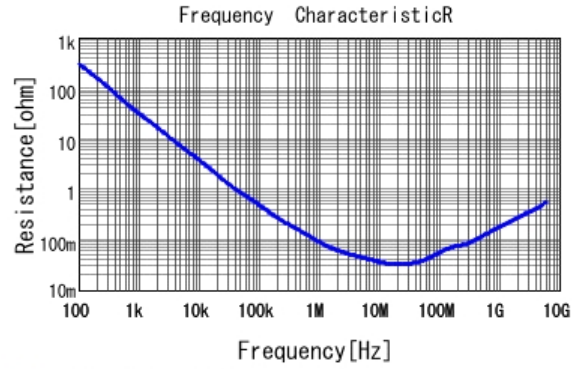
■ GRT033C81E104KE01 R DC0V, 25degC
