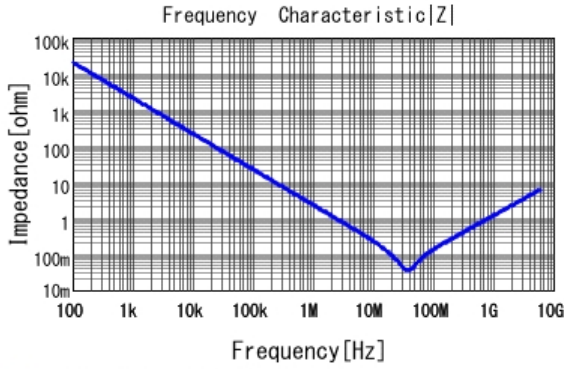
■ GRT033C81E104KE01 |Z| DC0V, 25degC
