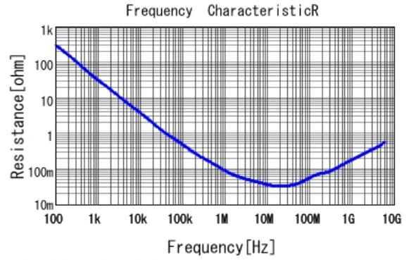
■ GRT033C81C104KE01 R DC0V, 25degC
