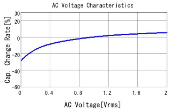
■ GRT033C81C104KE01 C-AC Voltage capchange, DC0V, 25.0d
