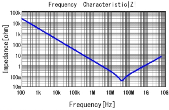
■ GRT033C81C104KE01 |Z| DC0V, 25degC
