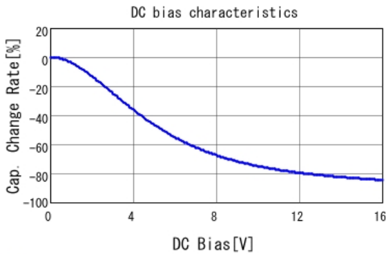
■ GRT033C81C104KE01 C-DC bias capchange, 25.0degC, AC1V
