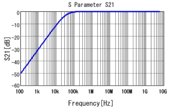
■ GRT033C80J473KE01 S21 DC0V, 25degC
