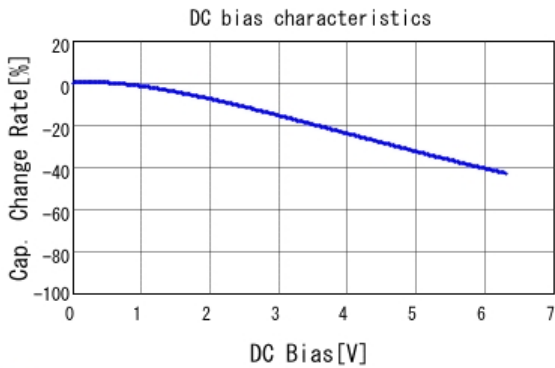
■ GRT033C80J473KE01 C-DC bias capchange, 25.0degC, AC0.
