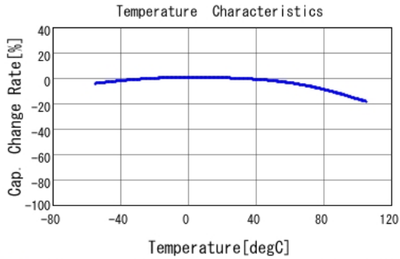
■ GRT033C80J473KE01 C-Temp. capchange, DC0.0V, AC0.5Vrm
