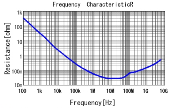
■ GRT033C80J473KE01 R DCOV, 25degC
