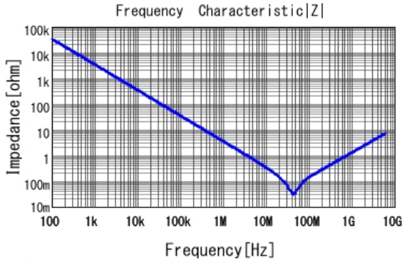
■ GRT033C80J473KE01 |Z| DCOV, 25degC
