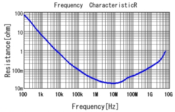
■ GRT033C80J224KE01 R DCOV, 25degC
