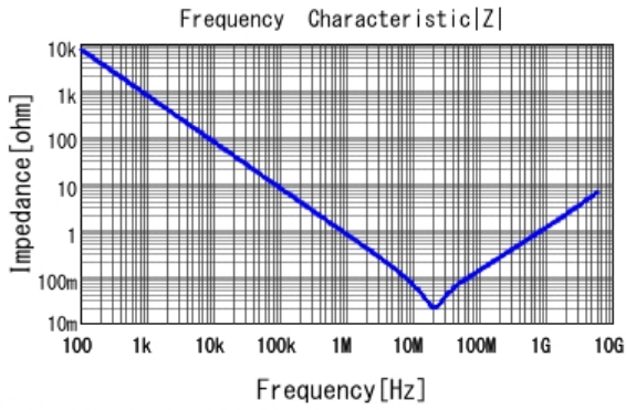
■ GRT033C80J224KE01 |Z| DCOV, 25degC
