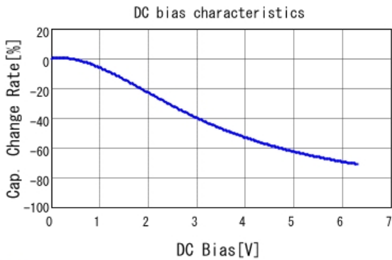
■ GRT033C80J224KE01 C-DC bias capchange, 25.0degC, AC0.
