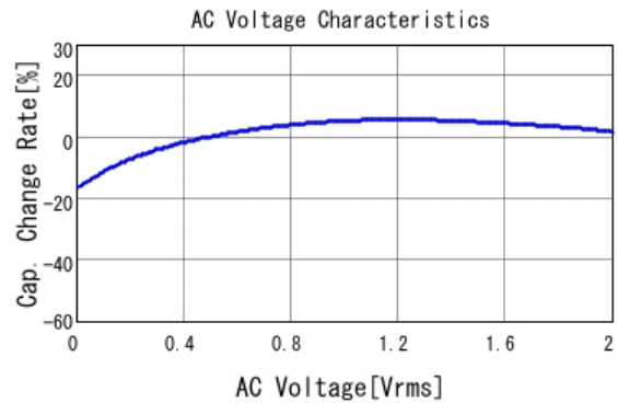
■ GRT033C80J224KE01 C-AC Voltage capchange, DCOV, 25.0d
