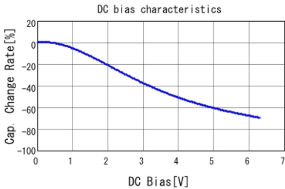
■ GRT033C80J105ME13 C-DC bias capchange, 25.0degC, AC0.
