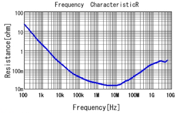
■ GRT033C80J105ME13 R DCOV, 25degC
