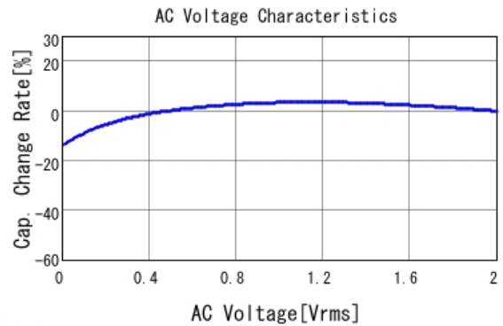
■ GRT033C80J105ME13 C-AC Voltage capchange, DCOV, 25.0d
