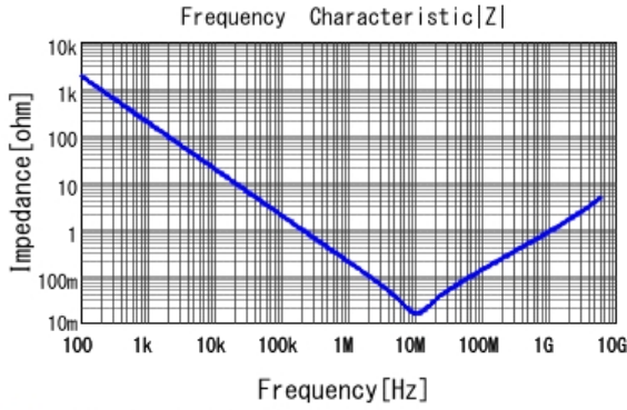
■ GRT033C80J105ME13 |Z| DCOV, 25degC
