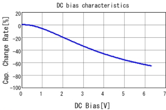
■ GRT033C80J104KE01 C-DC bias capchange, 25.0degC, AC0.
