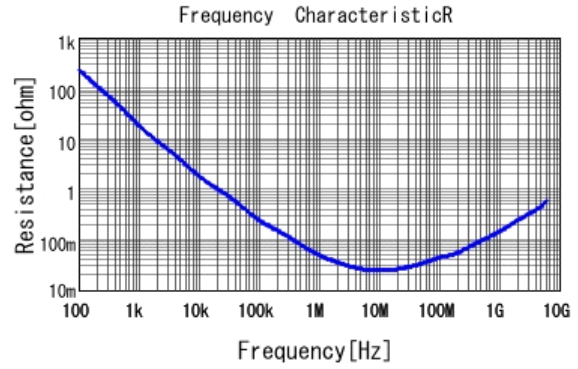
■ GRT033C80J104KE01 R DCOV, 25degC
