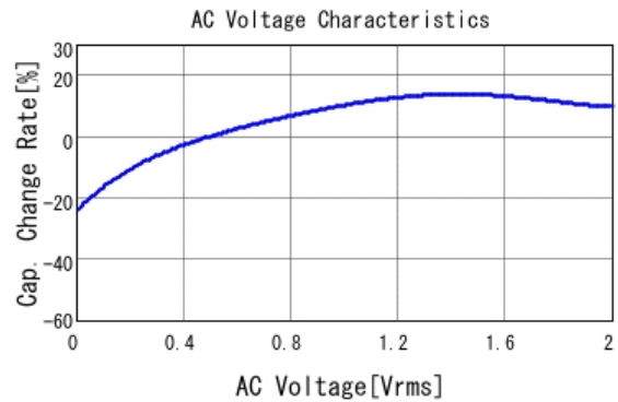
■ GRT033C80J104KE01 C-AC Voltage capchange, DCOV, 25.0d
