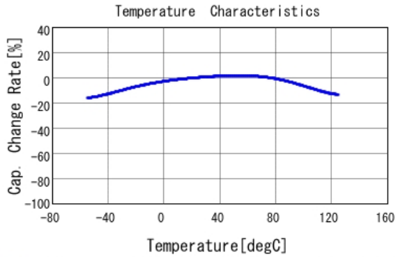
■ GRT033C70J104KE01 C-Temp. capchange, DC0.0V, AC0.2V rm
