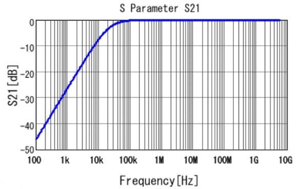
■ GRT033C70J104KE01 S21 DC0V, 25degC
