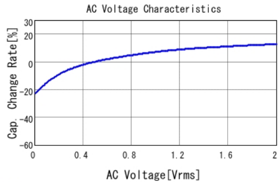
■ GRT033C70J104KE01 C-AC Voltage capchange, DC0V, 25.0d
