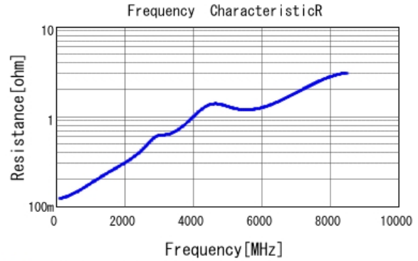
■ GRT0335C1H680JA02 R DCOV, 25degC
