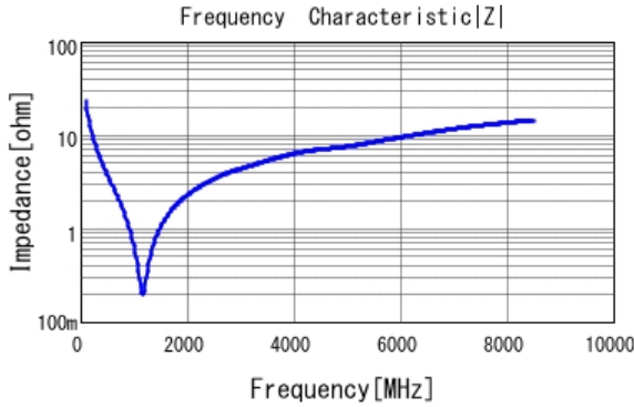
■ GRT0335C1H680JA02 |Z| DCOV, 25degC
