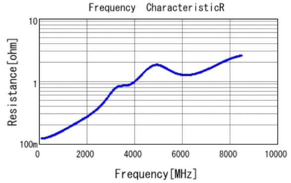
■ GRT0335C1H560JA02 R DCOV, 25degC
