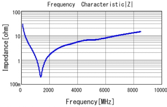
■ GRT0335C1H560JA02 |Z| DCOV, 25degC
