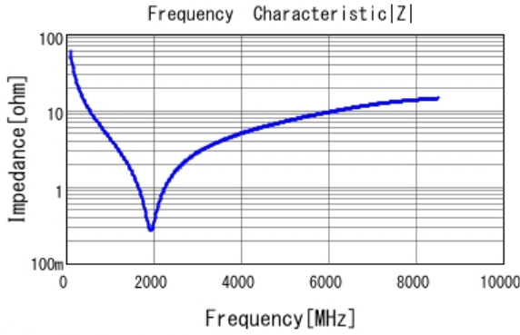
■ GRT0335C1H270JA02 |Z| DCOV, 25degC
