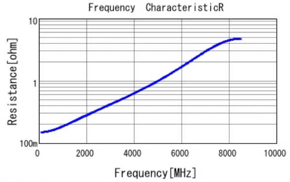
■ GRT0335C1H270JA02 R DCOV, 25degC
