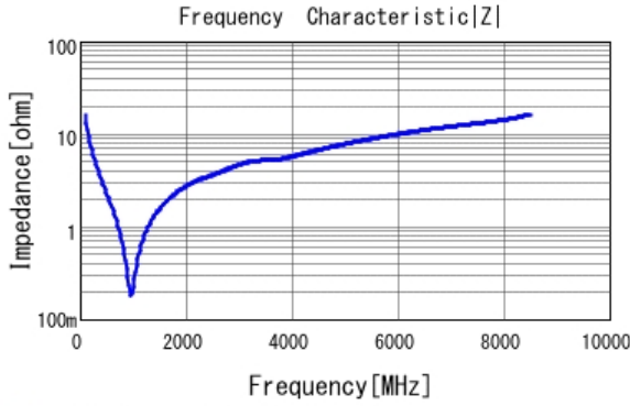
■ GRT0335C1H101JA02 |Z| DCOV, 25degC
