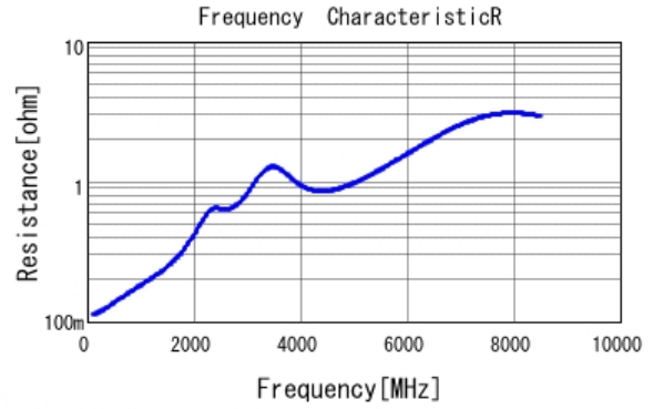
■ GRT0335C1H101JA02 R DCOV, 25degC
