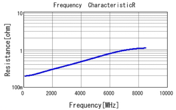
■ GRT0335C1H100JA02 R DC0V, 25degC
