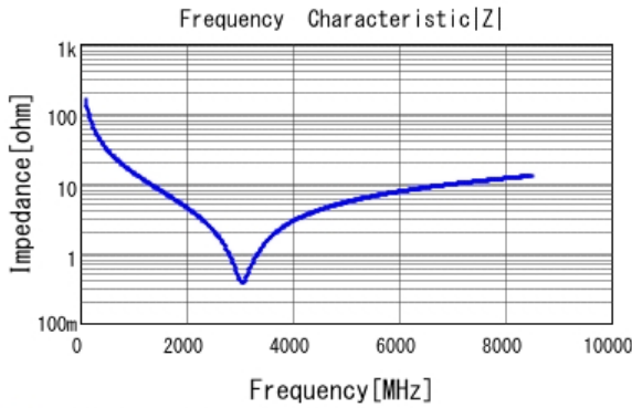
■ GRT0335C1H100JA02 |Z| DC0V, 25degC
