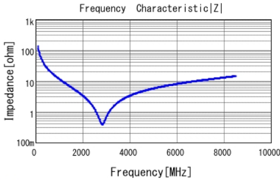
■ GRT0335C1E120FA02 |Z| DC0V, 25degC
