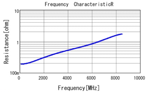
■ GRT0335C1E120FA02 R DC0V, 25degC
