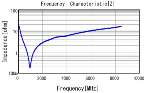
■ GRT0335C1E101JA02 |Z| DCOV, 25degC
