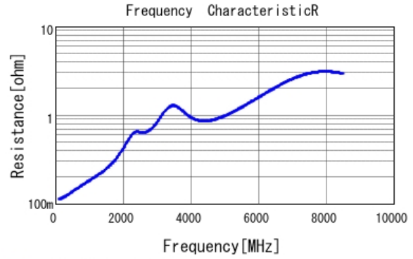
■ GRT0335C1E101JA02 R DCOV, 25degC
