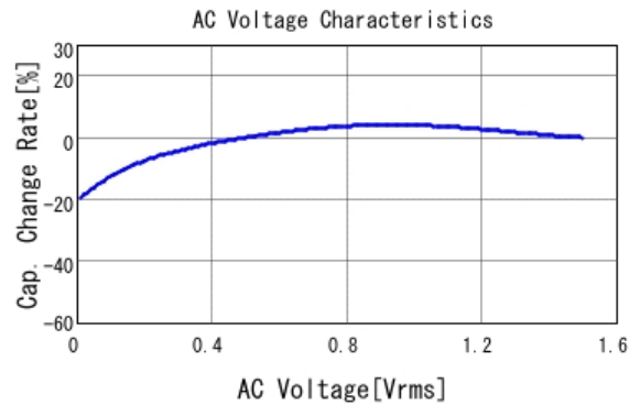
■ GRMJN7R61C226ME05 C-AC Voltage capchange, DCOV, 25.0d
