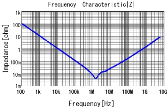
■ GRMJN7R61C226ME05 |Z| DCOV, 25degC
