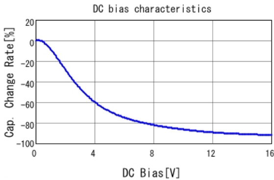
■ GRMJN7R61C226ME05 C-DC bias capchange, 25.0degC, AC0.
