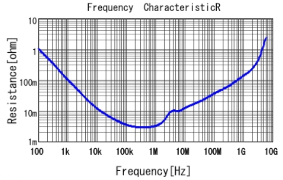
■ GRMJN7R61C226ME05 R DCOV, 25degC
