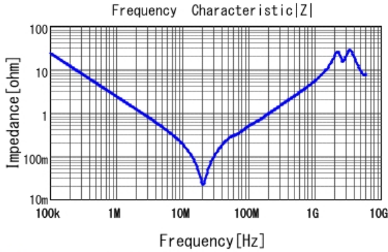
■ GRM55DR73A683KW01 |Z| DC0V, 25degC
