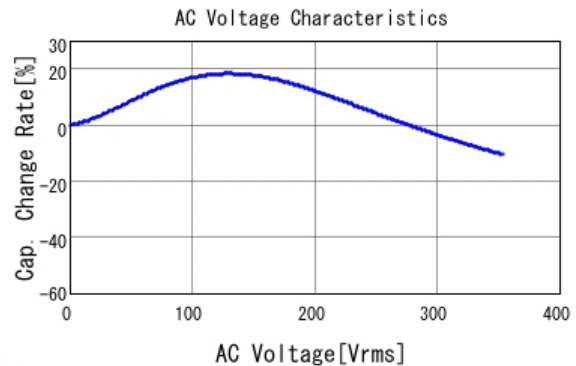
■ GRM55DR73A683KW01 C-AC Voltage capchange, DC0V, 25.0d
