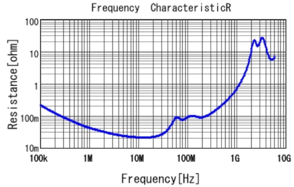
■ GRM55DR73A683KW01 R DC0V, 25degC
