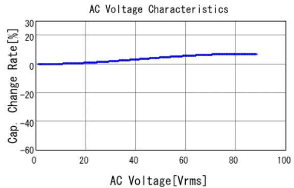
■ GRM55DR72E334KW01 C-AC Voltage capchange, DCOV, 25.0d
