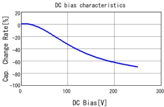
■ GRM55DR72E334KW01 C-DC bias capchange, 25.0degC, AC1V
