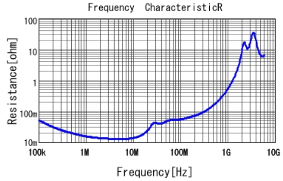
■ GRM55DR72E334KW01 R DCOV, 25degC
