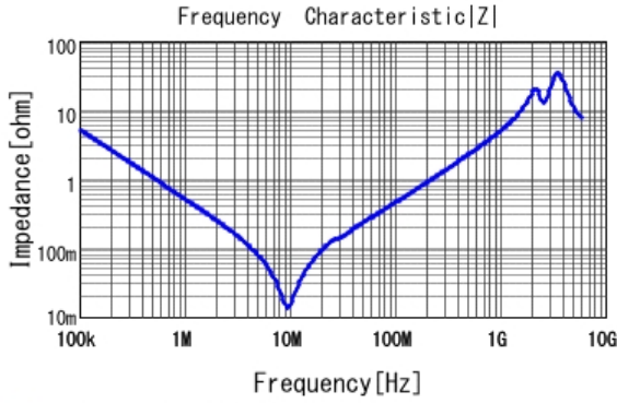
■ GRM55DR72E334KW01 |Z| DCOV, 25degC
