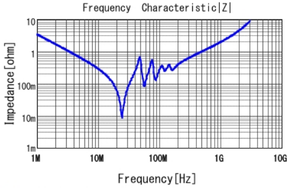
■ GRM55D7U2J473JW31 |Z| DC0V, 25degC
