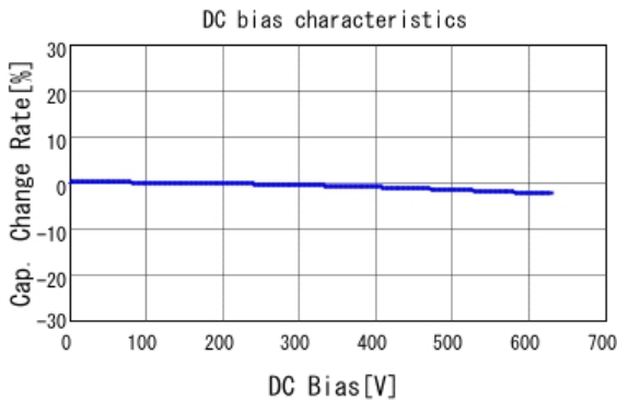
■ GRM55D7U2J473JW31 C-DC bias capchange, 25.0degC, AC1V
